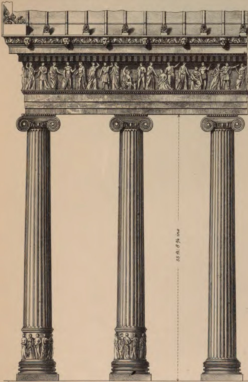
COLUMNS AND ENTABLATURE, WEST.
